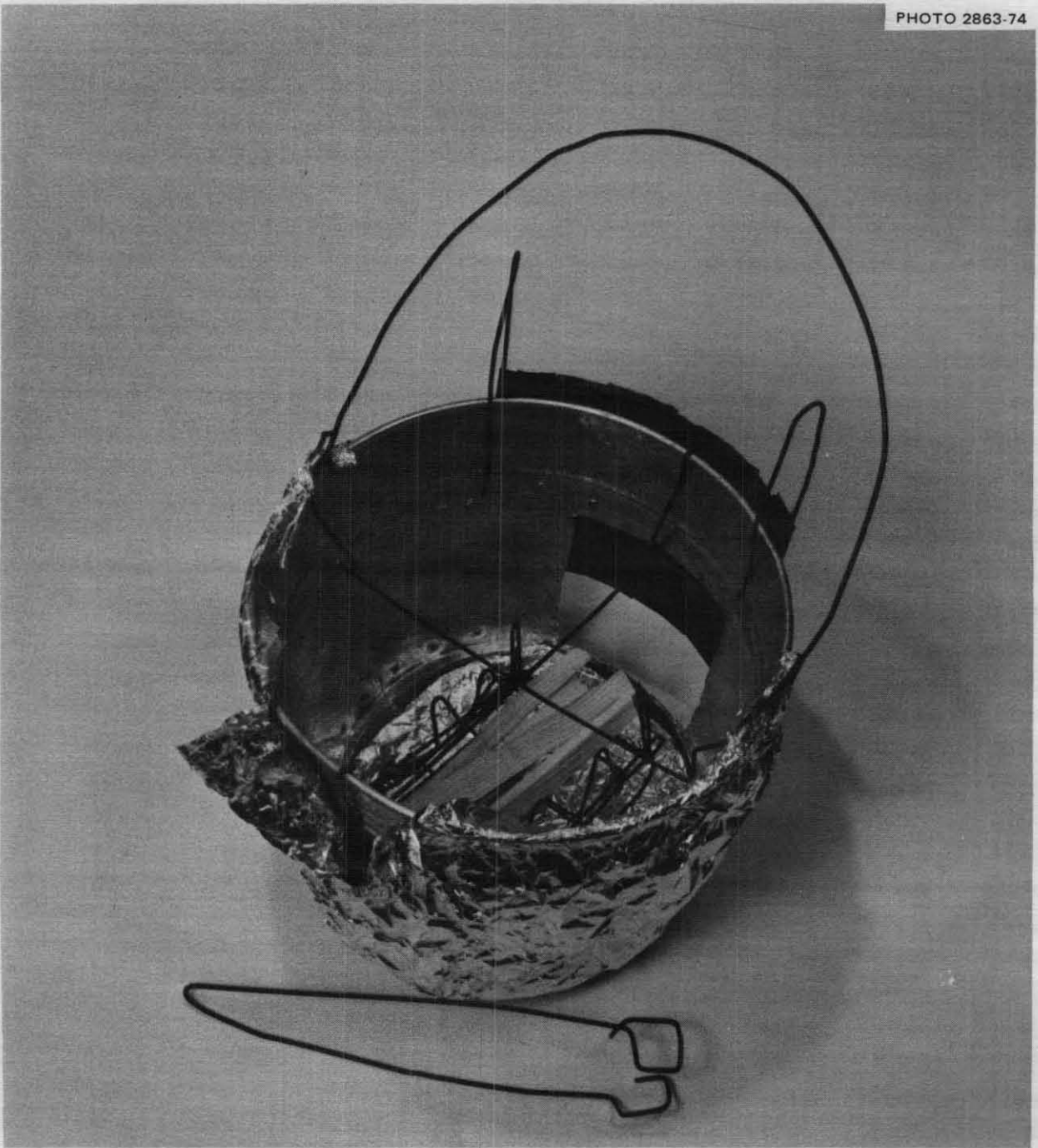
Fig. 37b. Bucket-Stove, showing its adjustable sliding damper partly closed, and the two coat-hanger wires that serve as pot supports. The ends of these wires are bent over the top of the bucket to form protruding springs to center and secure the pot by pressing against its sides. Pieces of wood about \frac{1}{2} \times \frac{3}{4} \times 6 in. are best.
